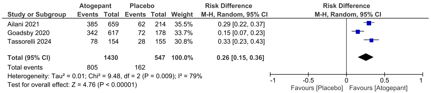
Supplementary Figure 3. Analysis of \geq 50\% reduction in monthly migraine days for combined atogepant dosages vs. placebo.
